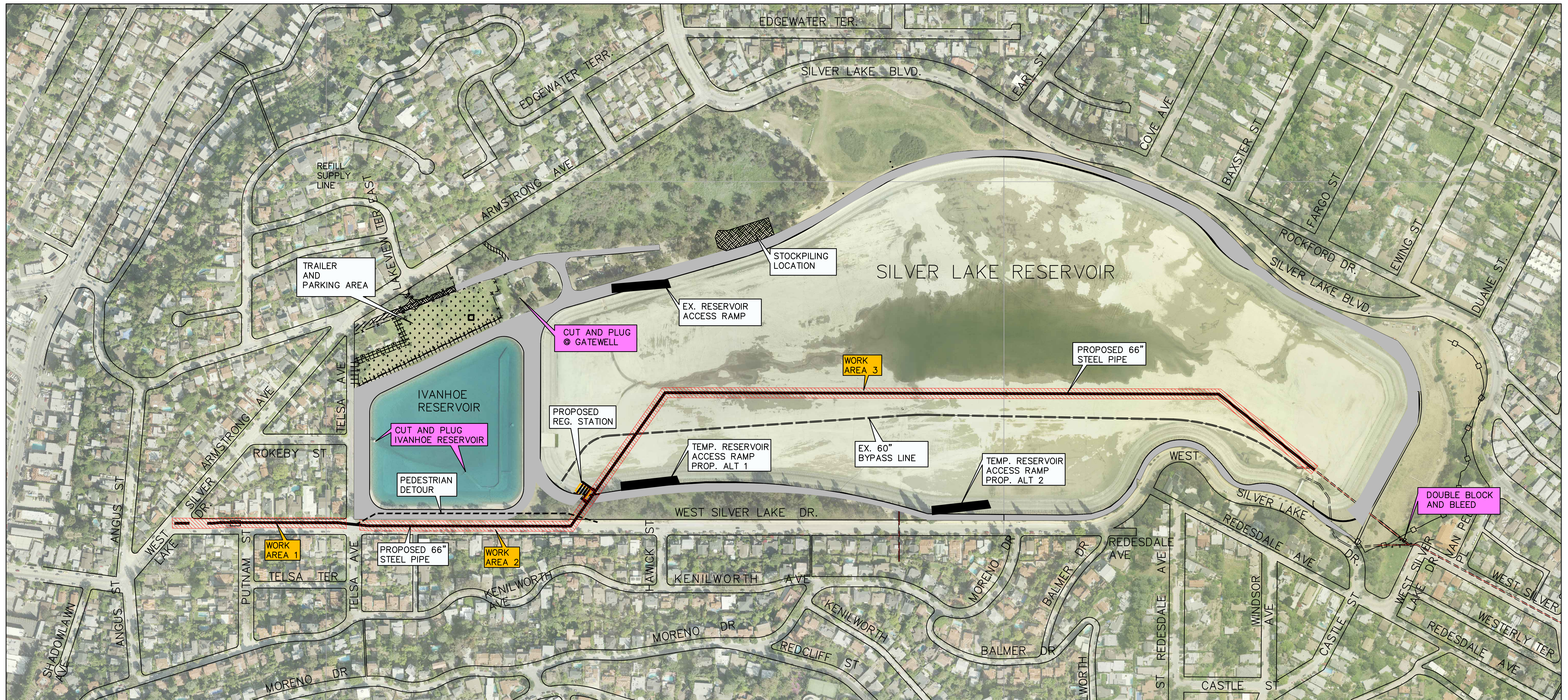
Silver Lake Reservoir Bypass Line and Regulator Station Project Overview Map
