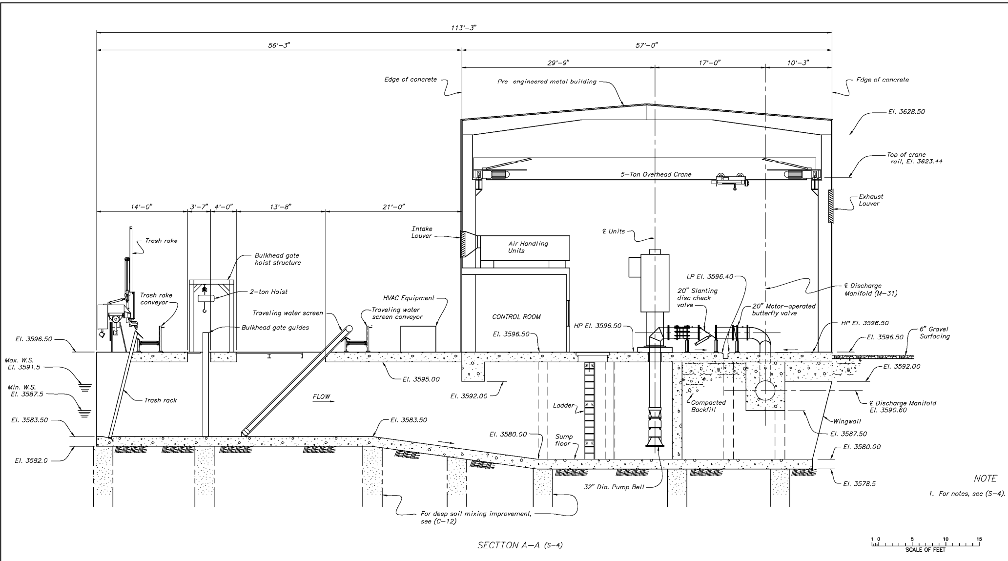
Figure 2-13. Side View of Pump Station
