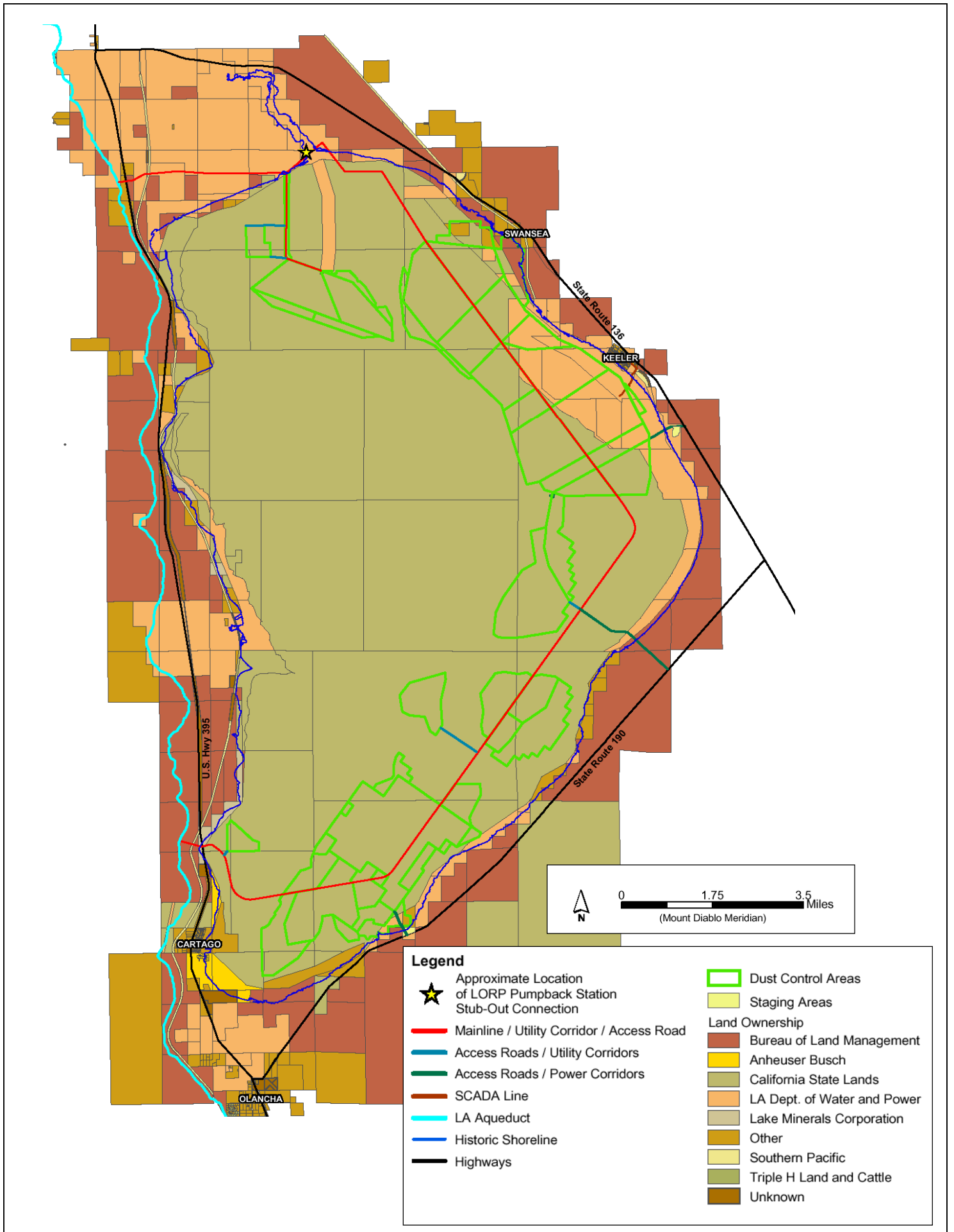
Figure 2-7A. Owens Lake Dust Control Project Facilities
