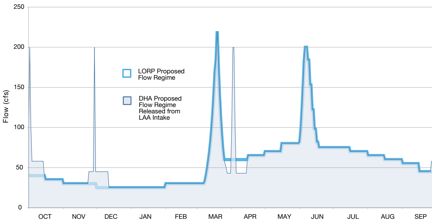
■ Figure 2. Proposed LORP Combined Flow Regime for River and Delta Habitat Area Flows released from the LAA Intake.
