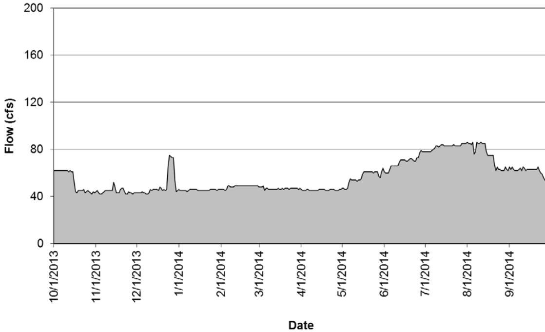
LORP at Mazourka Canyon Road Flow (Oct 13 to Sep 14)
