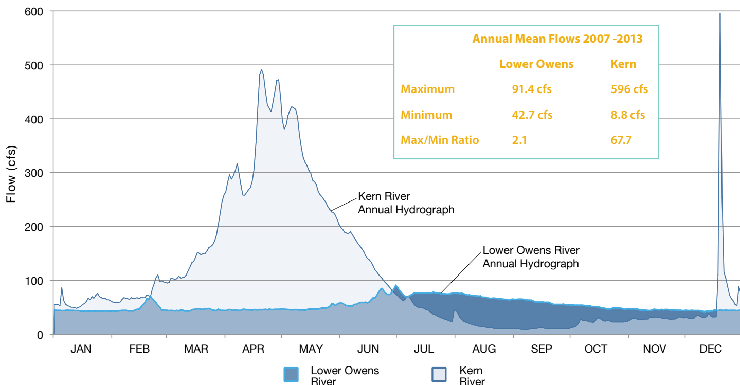
Hydrograph of mean daily flows for the Kern River and the Lower Owens River from 2007-2013. This comparison illustrates a natural hydrograph in the Kern River basin versus the artificial flow regime of the Lower Owens.
