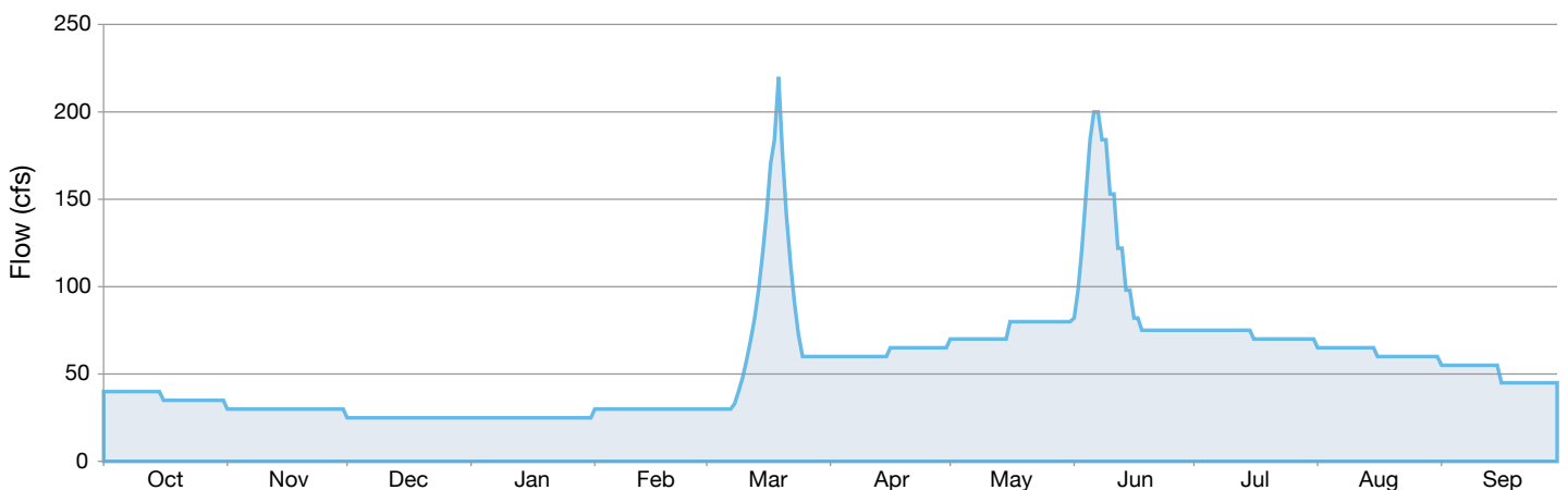
■ Figure 1. Proposed LORP Base and Seasonal Habitat Flow Regime at Intake release
