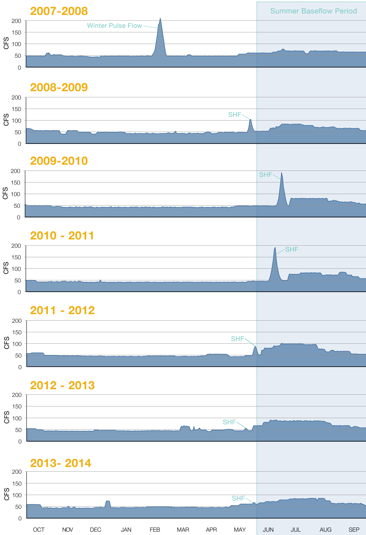
■ Annual hydrograph of the Lower Owens River from 2007-2014. These graphs illustrate the diminishing Seasonal Habitat Flows (SHF) through the years since the project was initiated with rewatering flows. It also illustrates the static flow regime and the abnormally high summer baseflows needed to meet the LORP Stipulation and Order of 40 cfs throughout the river system.
