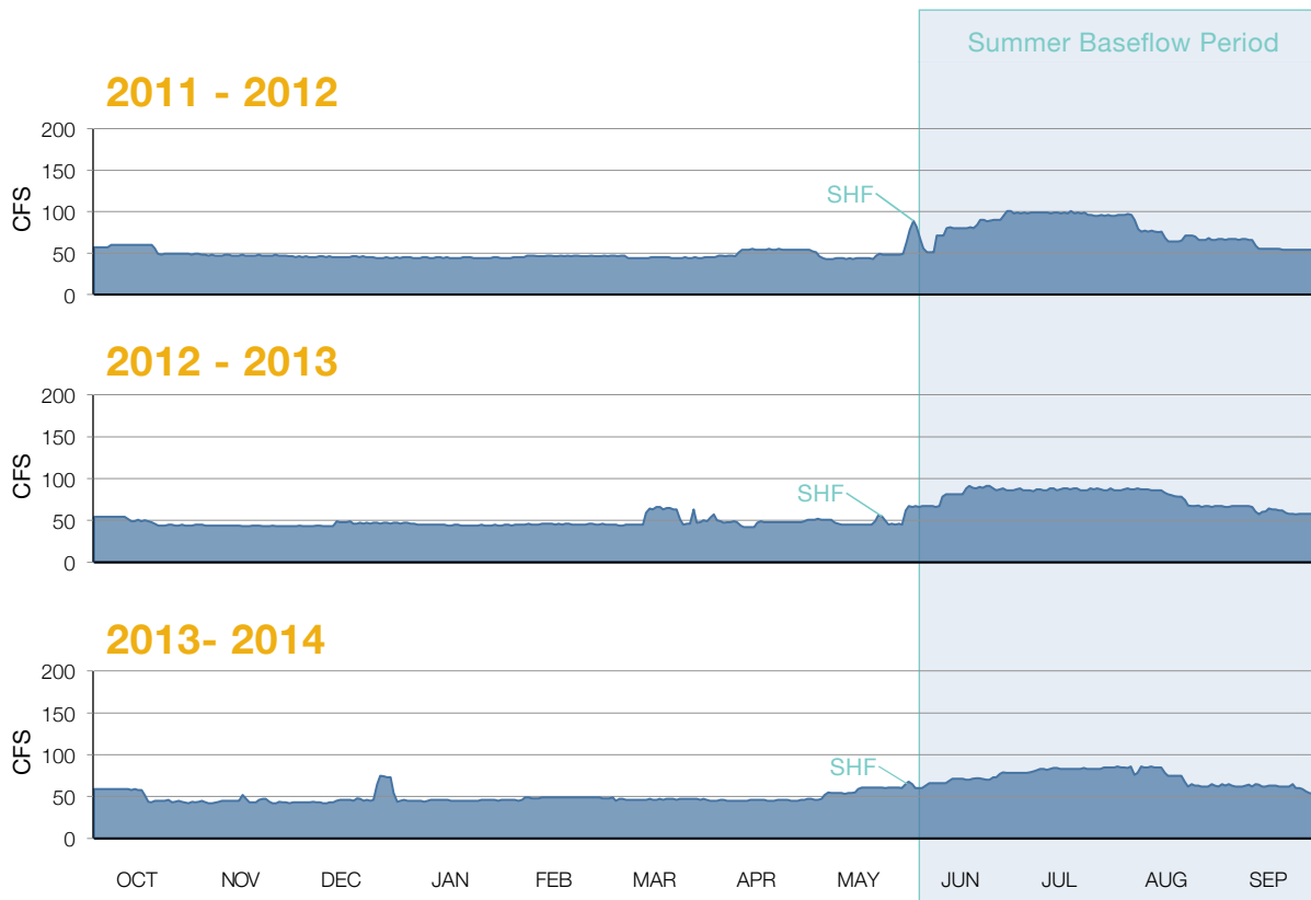
■ Figure 17. Annual hydrograph of the Lower Owens River from 2011-2014. These graphs illustrate the diminishing Seasonal Habitat Flows (SHF) through the years since the project was initiated with rewatering flows. It also illustrates the static flow regime and the abnormally high summer baseflows needed to meet the LORP Stipulation and Order of 40 cfs throughout the river system.
