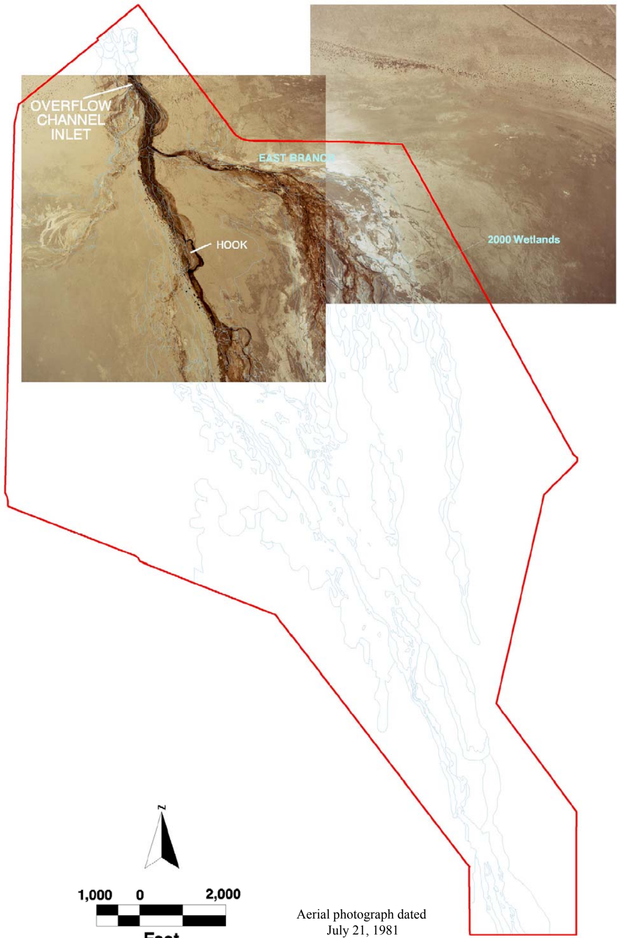
Figure 6-7. Delta Habitat Conditions in 1981
