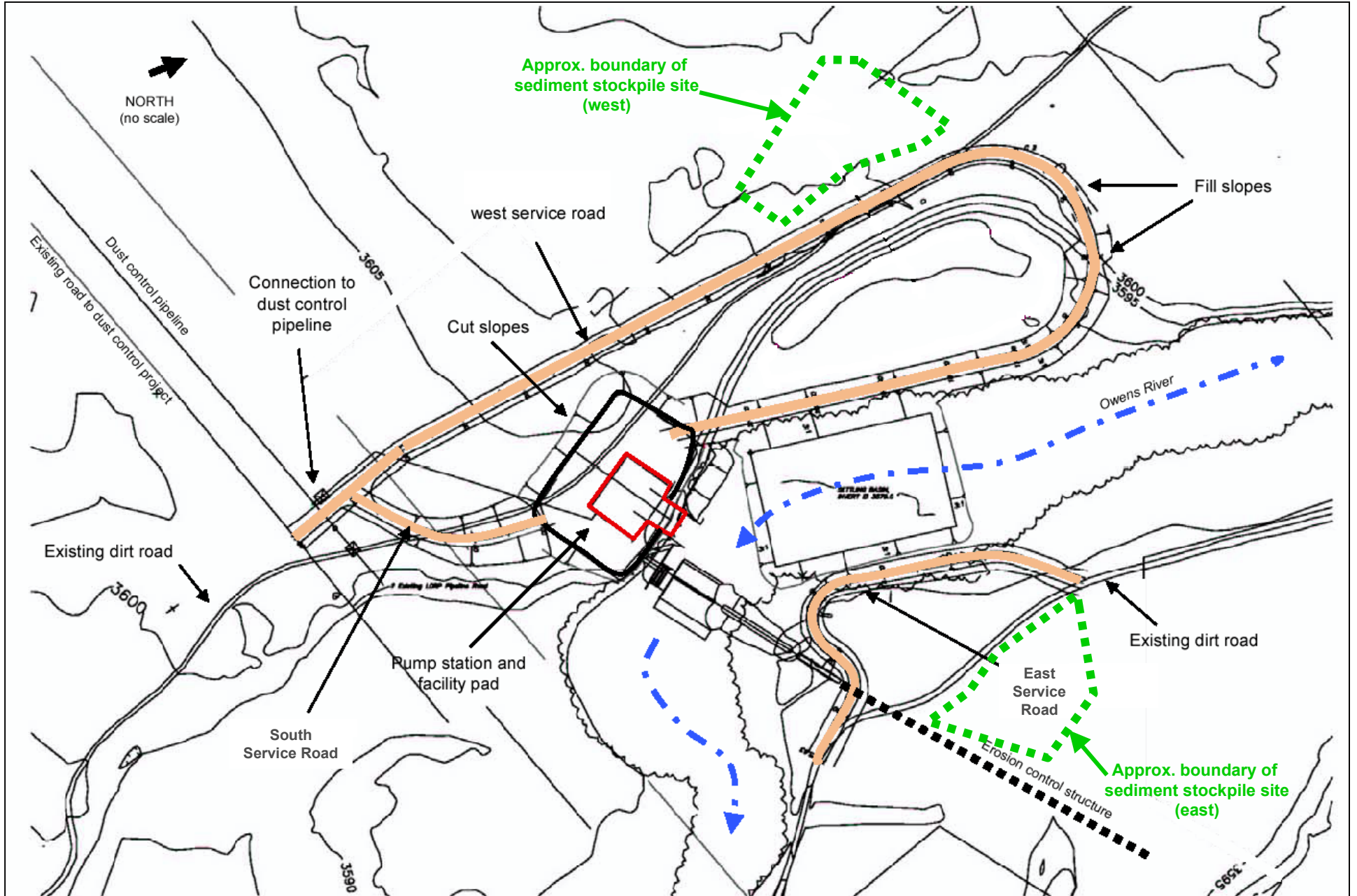
Figure 2-9. Service Roads at the Pump Station
